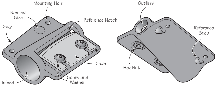
Figure 1: Dowel and tenon cutter components.
