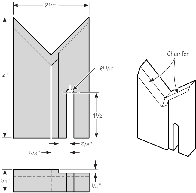
Figure 5: Outfeed support V-block (adjustable).
