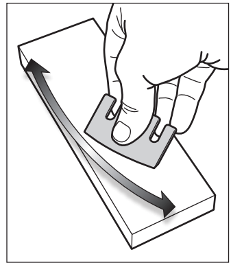
Figure 15: Honing.
