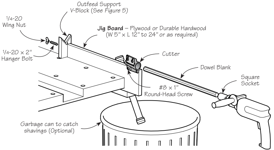
Figure 3: Alternative dowel-making set-up.
