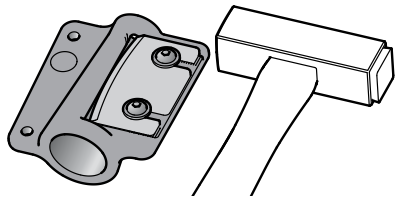
Figure 13: Blade adjustment.
