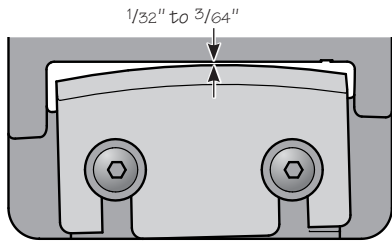
Figure 12: Blade placement.
